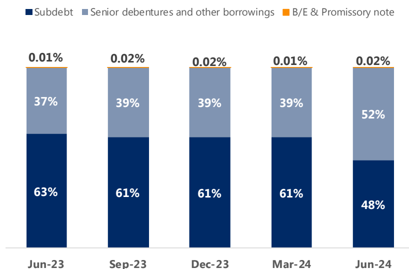
Figure 20: Borrowings breakdown
