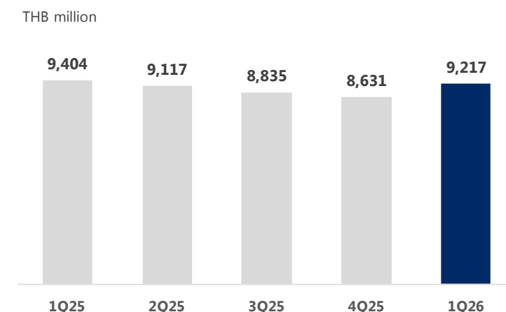
Figure 8: Pre-provision operating profit (PPOP)
